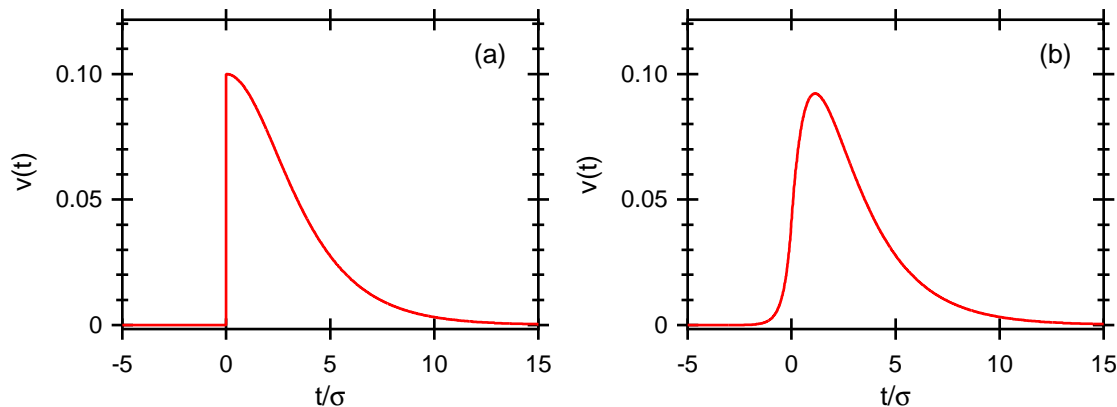
FIG. 4: Graph of v(t) versus t/\sigma for an impulsive force ( \eta = 0.25 , v_0 = 0.1 ). (a) Exact equation of motion (50). (b) Approximate integro-differential equation of motion (69) with N = 4 .
