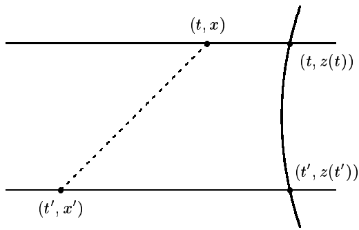
FIG. 3: Spacetime diagram, which illustrates a pair of events (t, x) and (t', x') that give a nonzero contribution to \bar{F}_r(t, t') . The thick solid line indicates the particle trajectory, the thin solid lines indicate the planes of simultaneity for times t and t' , the dashed line indicates the light-like interval between events (t', x') and (t, x) .
