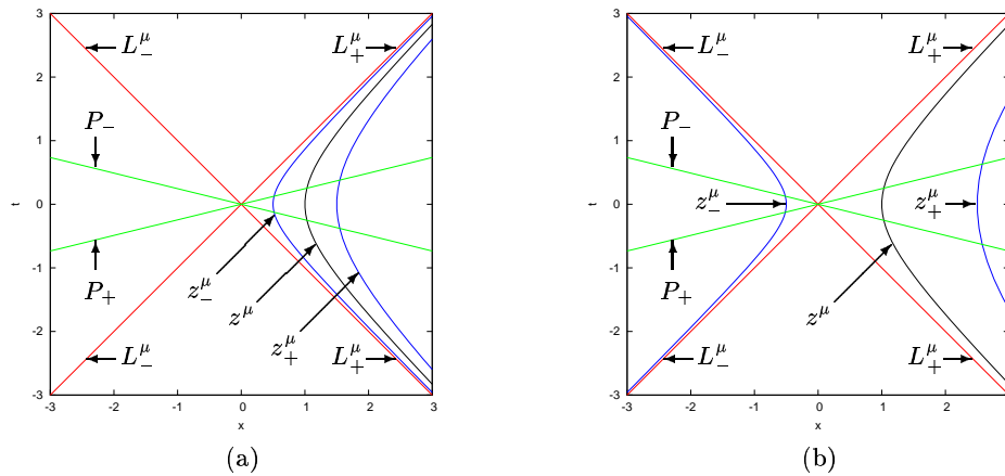
FIG. 2: Spacetime diagrams for a uniformly accelerated particle of radius R . Black curve: particle trajectory z^\mu . Blue curves: trajectories z_-^\mu and z_+^\mu of the left and right edges of the particle. Red curves: trajectories L_+^\mu and L_-^\mu . Green curves: planes of simultaneity P_\pm for \tau = \pm 1/4 . (a) aR = 1/2 . (b) aR = 3/2 .
