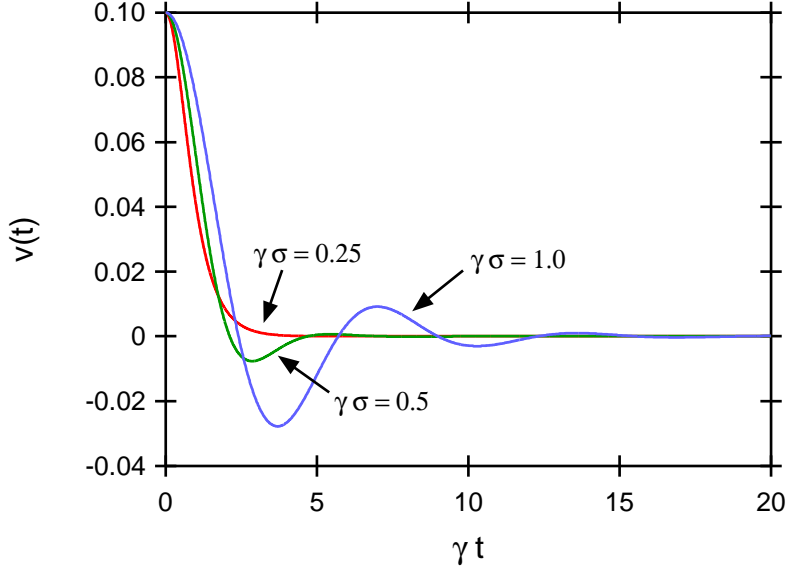
FIG. 5: Graph of v(t) versus \gamma t for an impulsive force ( v_0 = 0.1 ). Red curve: \gamma\sigma = 0.25 . Green curve: \gamma\sigma = 0.5 . Blue curve: \gamma\sigma = 1.0 .
