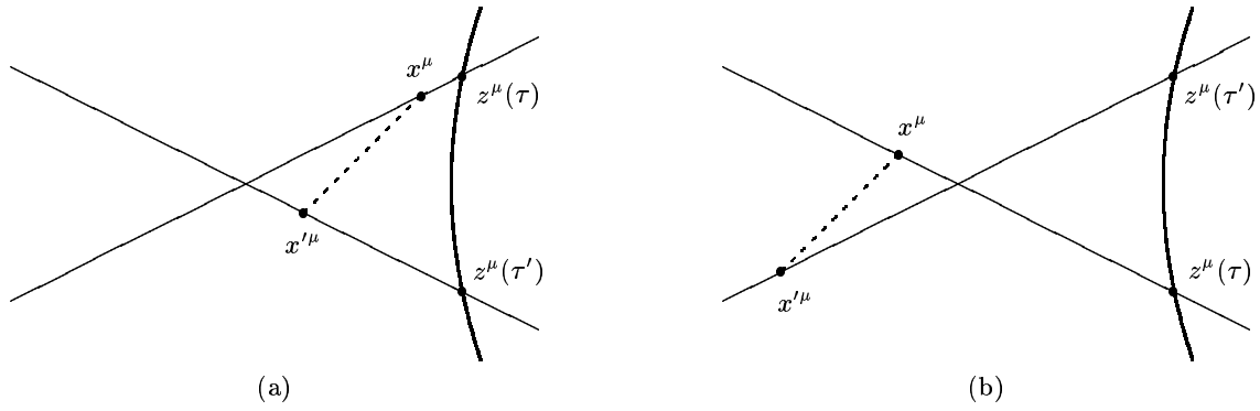
FIG. 1: Spacetime diagrams, which illustrate pairs of events x^\mu and x'^\mu that give nonzero contributions to \bar{K}_r^\mu(\tau, \tau') . The thick solid lines indicate the particle trajectory, the thin solid lines indicate the planes of simultaneity for proper times \tau and \tau' , the dashed lines indicate the light-like interval between events x^\mu and x'^\mu . (a) Conditions (1–3) are satisfied for \tau > \tau' , corresponding to retarded effects. (b) Conditions (1–3) are satisfied for \tau < \tau' , corresponding to advanced effects.
