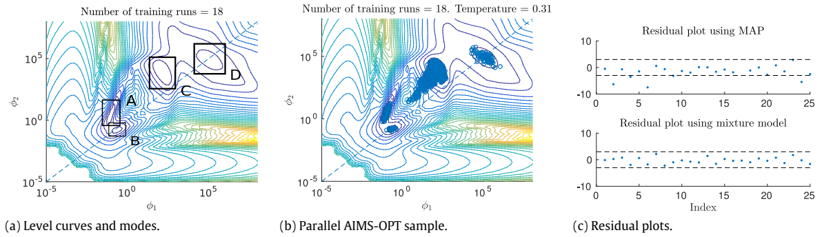
Fig. 4. Projection of the negative log-posterior curves in the two dimensional length-scale space for the Branin simulator. The minimum possible value of 10^{-12} for the nugget \phi_\delta has been used for such projection. The reference diagonal helps visualise the regions where the length scales favour one dimension over the other.
