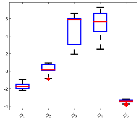
Fig. 6. Box-plots of the sample of length-scales obtained by the parallel asymptotically independent Markov sampling. (For interpretation of the references to colour in this figure legend, the reader is referred to the web version of this article.)
