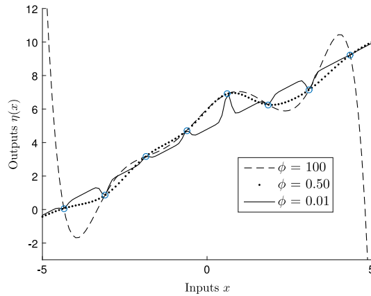
Fig. 1. The length-scale parameters represent how sensitive is the output of the simulator to variations in each dimension. The plot corresponds to 8 design points chosen for the function \eta(x) = 5 + x + \cos(x) + 0.5 \sin(3x) . For low values of the length-scale parameter the training runs are less dependent of each other.
