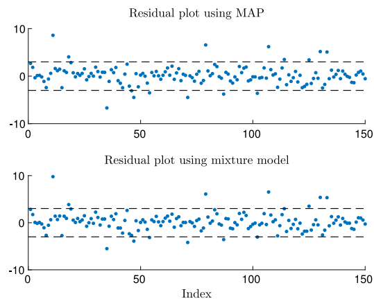
Fig. 7. Residuals plot for the Nilson-Kuusk simulator.
