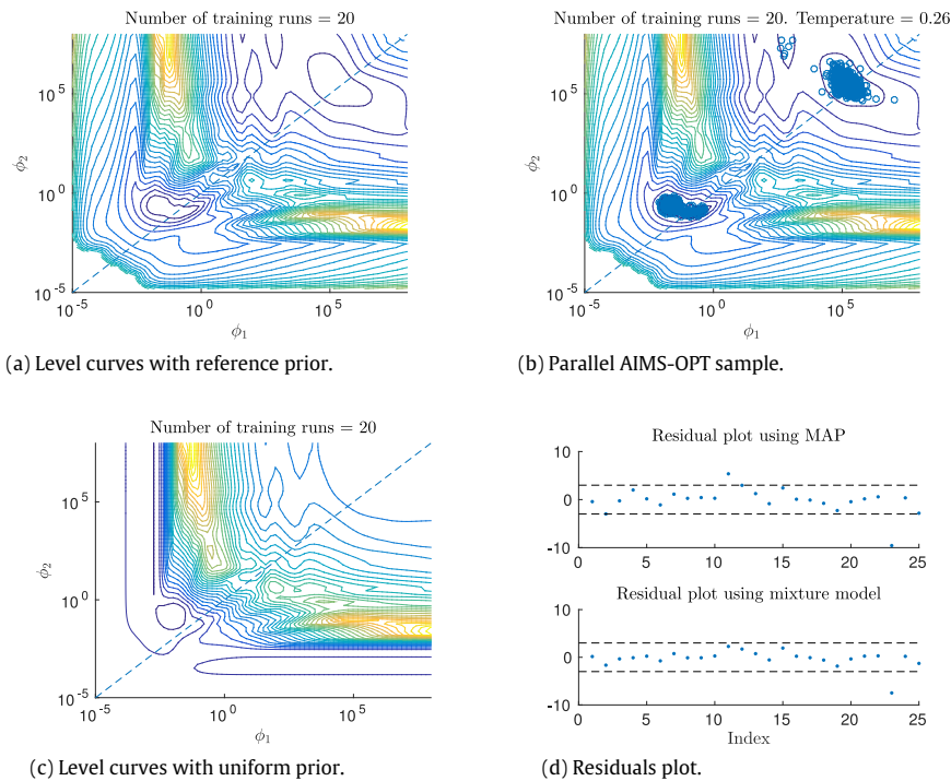
Fig. 5. Projection of the negative log-posterior curves in the two dimensional length-scale space for the 2D Model simulator. The minimum possible value of 10^{-12} for the nugget \phi_8 has been used for such projection. The reference diagonal helps visualise the regions where the length scales favour one dimension over the other.
