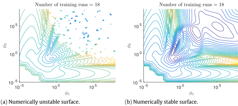
Fig. 3. Projection of the negative log-posterior curves in the two dimensional length-scale space. Adding the nugget \phi_\delta results in a numerically stable surface.
