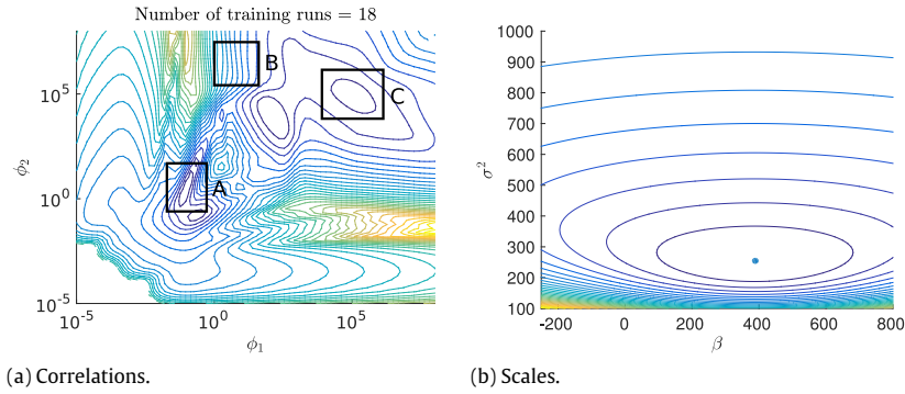
Fig. 2. In 2(a), different dynamics of the hyper-parameters for the log-posterior distribution of a test function (see Section 5.1) are shown: A. corresponds to positive correlation. B. corresponds to an independent region. C. corresponds to negative correlation. In 2(b), the marginal log-posterior function of the same example with h(\mathbf{x}) = 1 , presents the same contour level for a wide range of \beta . Thus, the hyper-parameters exhibit very different scales. The dot represents the minimum of the corresponding function.
