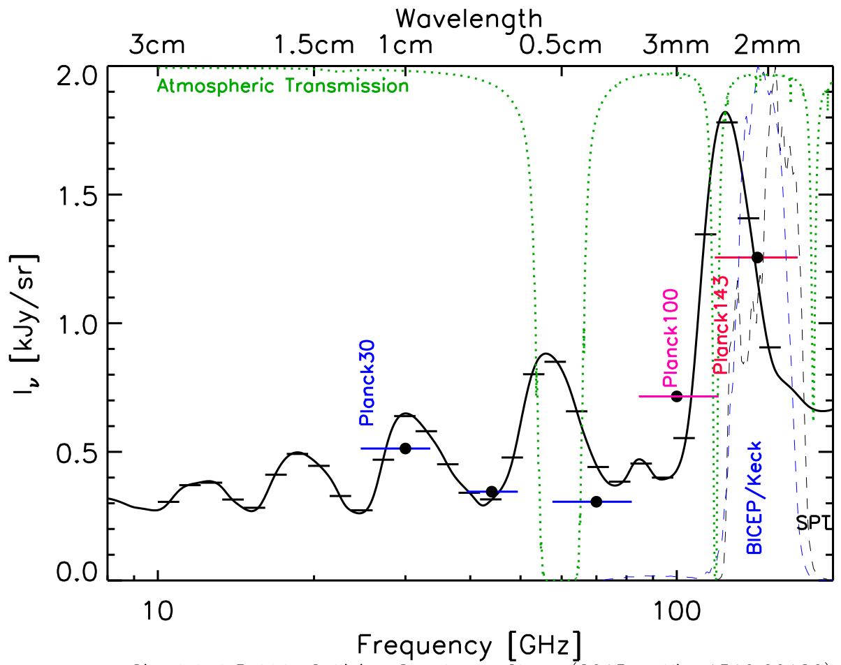
Simulated Bubble Collision Spectrum: Chary (2015; arXiv: 1510.00126)
