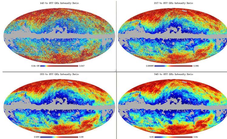
Fig. A.1.— All-sky maps in Galactic Mollweide projection at NSIDE=2048 (1.8') resolution showing the ratio of intensity at a particular frequency to the 857 GHz intensity. As can be seen, higher Galactic latitudes tend to have cooler ISM emission and thereby higher ratios, than regions close to the Galactic Plane which has been masked as described in the text.
