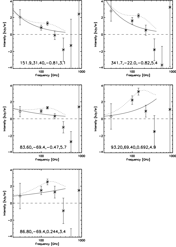
Fig. B.5.— The five panels show as stars the spectrum of emission in the five regions in Table 2. Also shown (diamond) is the residual 30 GHz intensity from the Planck LFI maps of the same resolution. The solid line is the best fit to the 30, 100 and 217 GHz points with the four numbers at the bottom left being (l, b, \alpha, SNR_{excess,143}) where \alpha is the spectral index of the fit and SNR_{excess,143} is as defined in Table 3. While the 3\sigma points have a random probability of occurring a handful of times in a map with 12000 pixels, the \gtrsim 5\sigma points should occur only once in 70 maps and the 5.7\sigma point once in 70000 maps. The dotted line shows the result of adding a continuum black body component of 2.7K, which may be due to residual CMB or ISM; the measurements at 100 and 217 GHz are clearly violated, arguing that the excess is more likely due to line emission.
