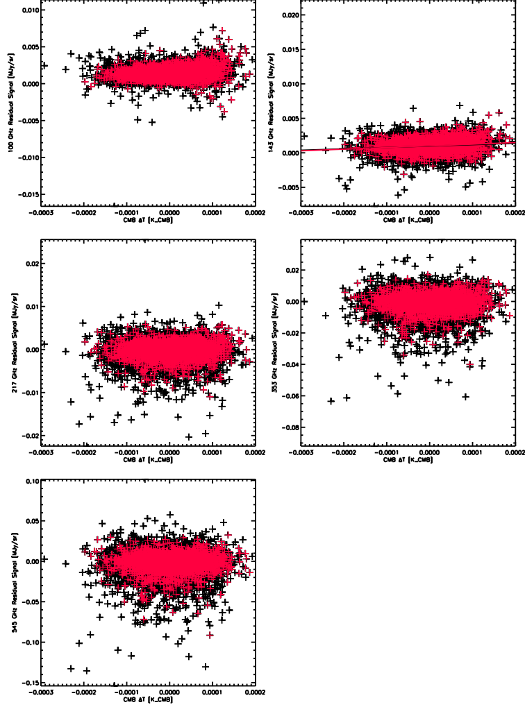
Fig. B.3.— Residual emission at each of the frequencies shown against the CMB temperature decrement. The black points are each pixel in the 1.8^\circ resolution maps with \text{ISM} < 8 \text{ MJy/sr} . The red points are only the ones with \text{ISM} < 4 \text{ MJy/sr} and at Galactic latitudes greater than 45^\circ . Except for 100 and 143 GHz, the median of the residuals at each frequency is consistent with zero.
