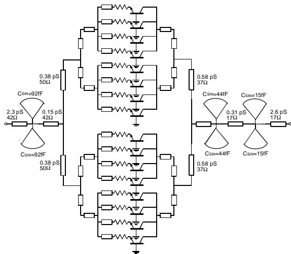
Figure 2 DHBTT MMIC power amplifier in transferred-substrate technology
