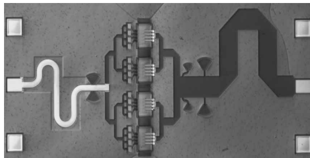
Figure 3 Die photograph of MMIC power amplifier in transferred-substrate technology
